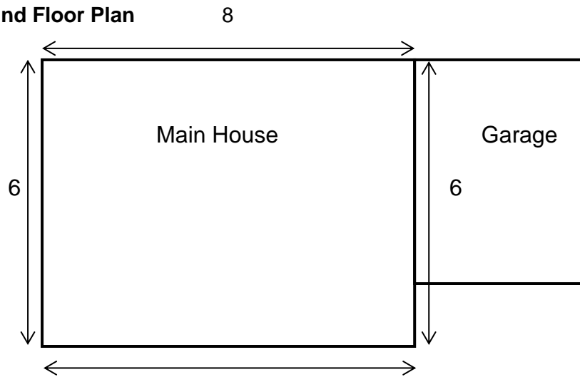
Figure N3: Areas and perimeters for two storey detached house with extension over garage. The floor over the garage a semi-exposed timber floor
