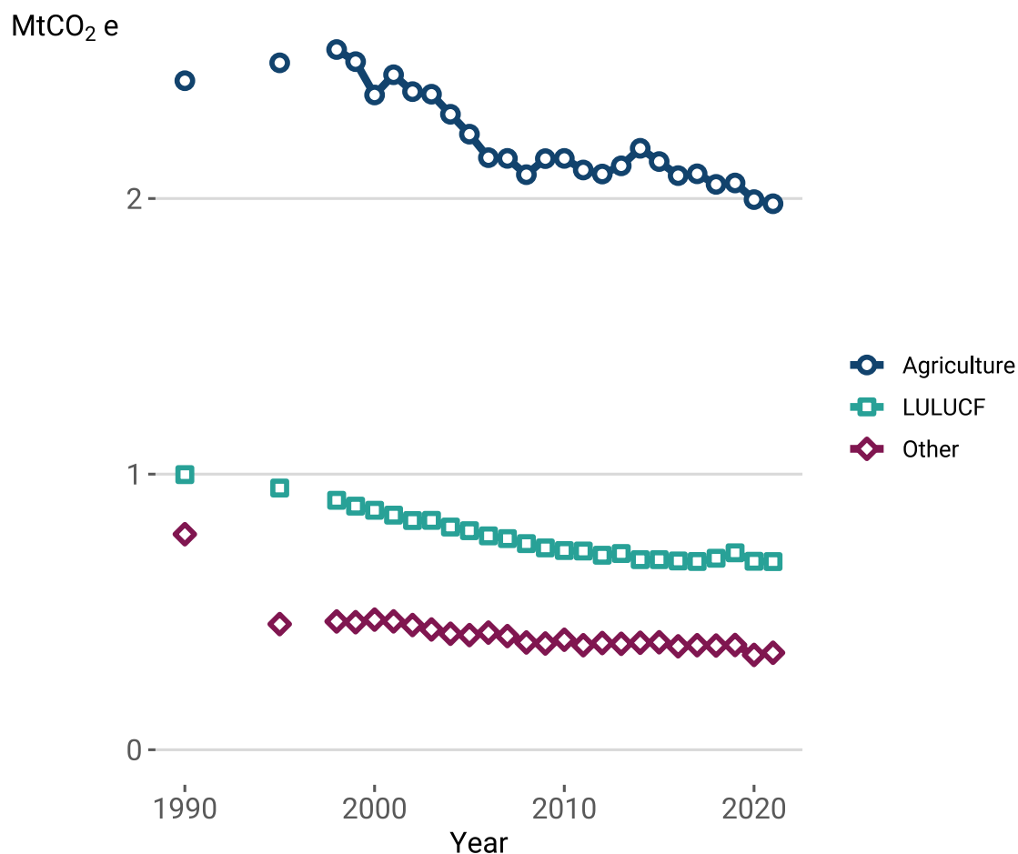
Chart 13. Nitrous Oxide (N 2 O) Emissions by National Communications Category, 1990 to 2021.
