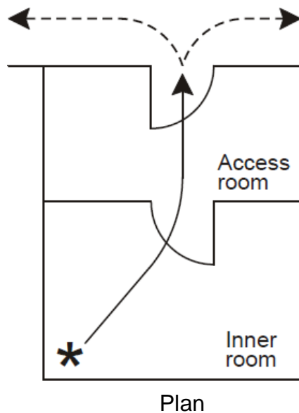
Figure 6 Single direction of escape out of an inner room and through an access room before a choice of escape routes becomes available
