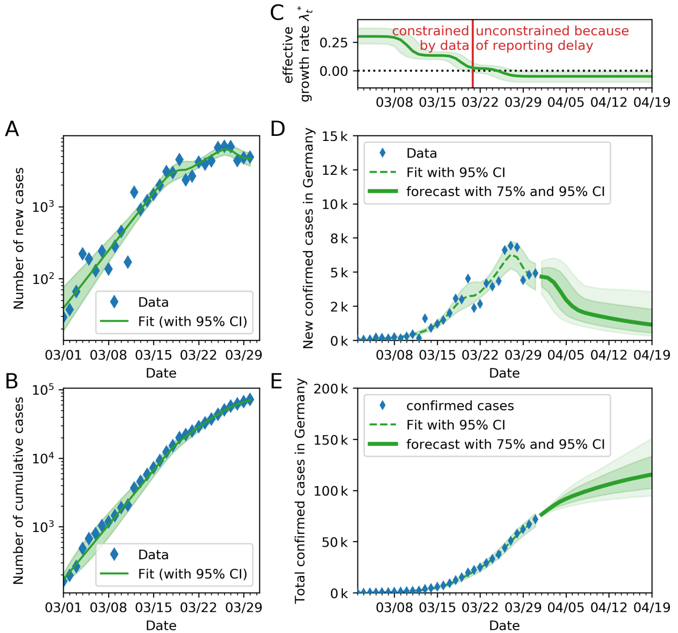
FIG. S3. Inferring and forecasting (the time of) the change point in spreading rate \lambda , assuming three change points . Please refer to Fig. 3 for the case with two change points. A: Comparison of daily recorded new cases and the model, log scale. B: Comparison of total recorded cases and the model, log scale. C: Time-dependent model-estimate of the spreading rate \lambda_t . D: Model forecast of new cases, based on the inferred \lambda_t , linear scale. E: Model forecast of total cases, based on the inferred \lambda_t , linear scale.
