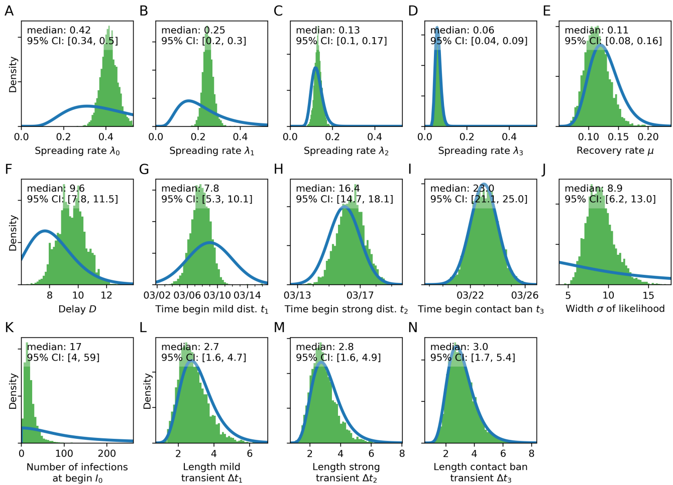
FIG. S4. Posterior distributions from the change-point detection with three change points (green) compared to prior distributions (blue). Please refer to Fig. 4 for a more detailed description of the distributions.
